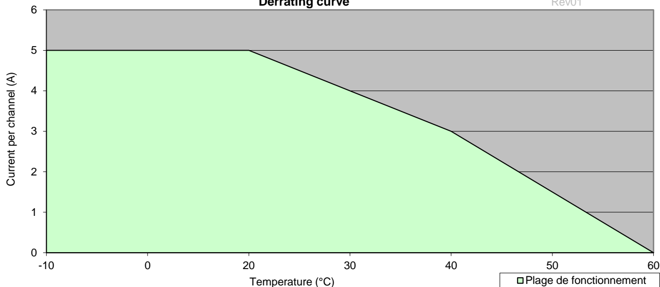
Derrating curve
